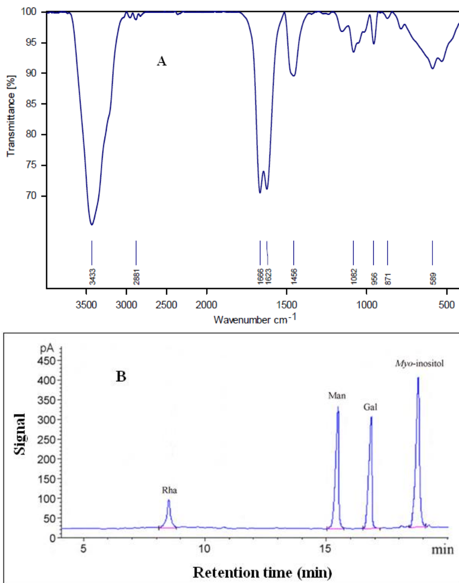
Figure 5. A) FT-IR spectrum and B) Gas chromatogram analysis of monosaccharide composition.
