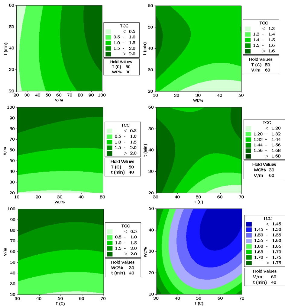
Figure 4. Contour plots of TCC vs. extraction variables.
