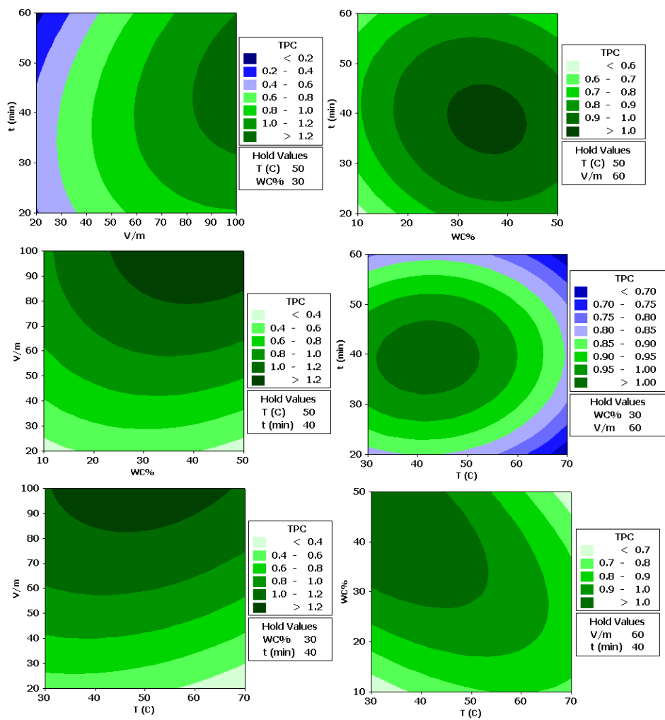
Figure 7. Contour plots of TPC vs. extraction variables.
