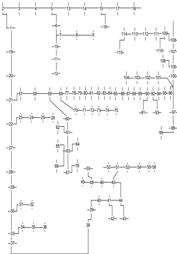
Fig. 3. Single Linear 115-Bus Diagram of Tabriz.
