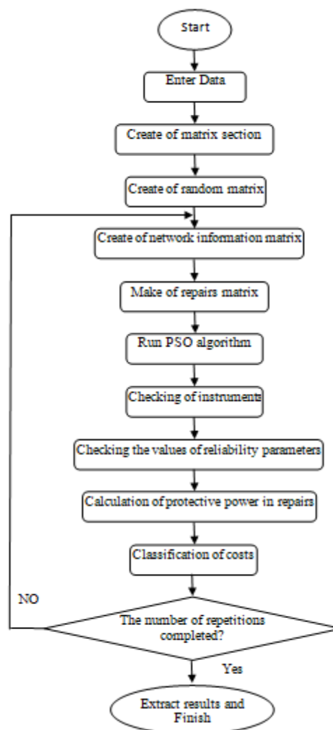
Fig. 2. Flowchart of executing the program.
