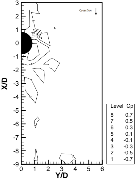
Figure 13: Surface distribution around the nozzle exit ( \beta=90, \alpha=75 )
