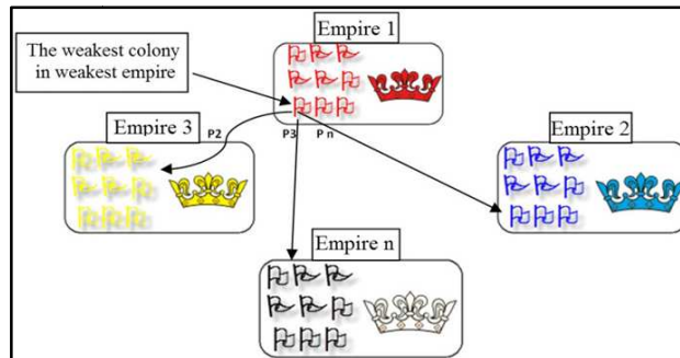
Figure4. Imperialistic competition: The more powerful an empire is, the more likely it will possess the weakest colony of the weakest empire
