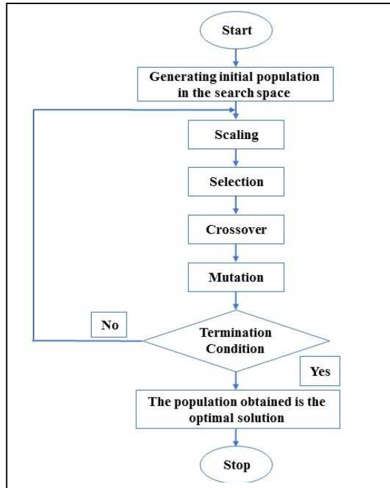
Figure1. Genetic algorithm flow chart
