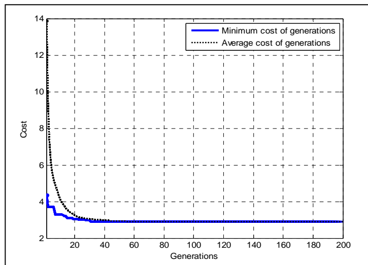
Figure9. Convergence of the objective of minimum cutting time for GA
