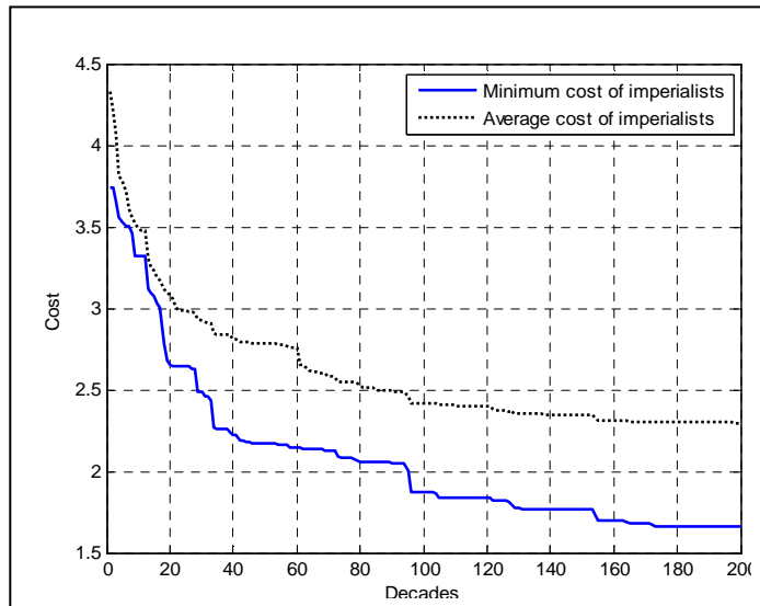
Figure8. Convergence of the objective of minimum cutting time for CCA
