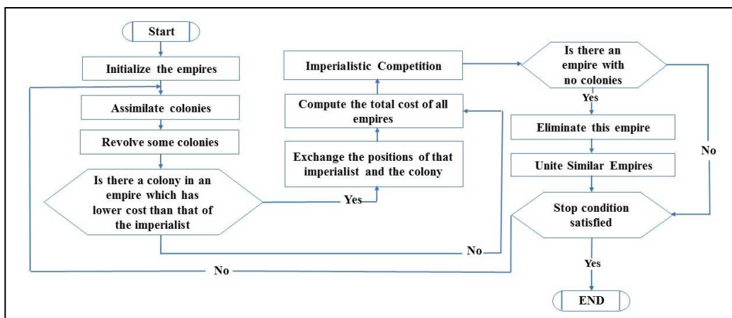
Figure5. Flowchart of the Colonial Competitive Algorithm
