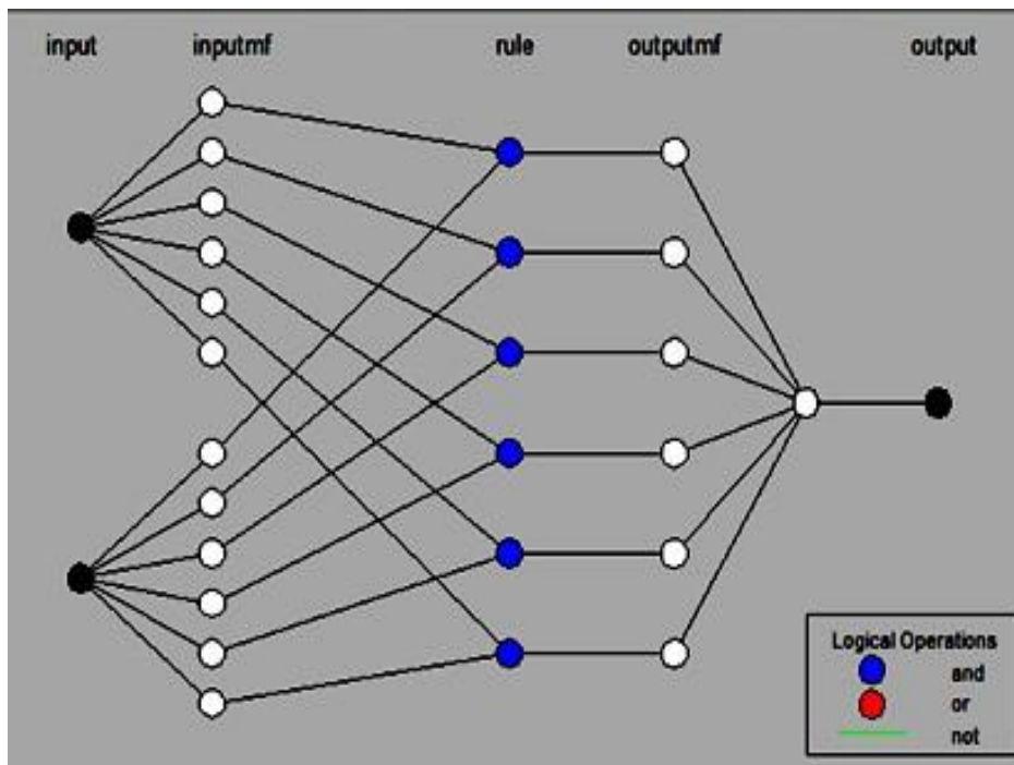
Figure5. The structure of ANFIS using6fuzzy sets designed inMatlab software
