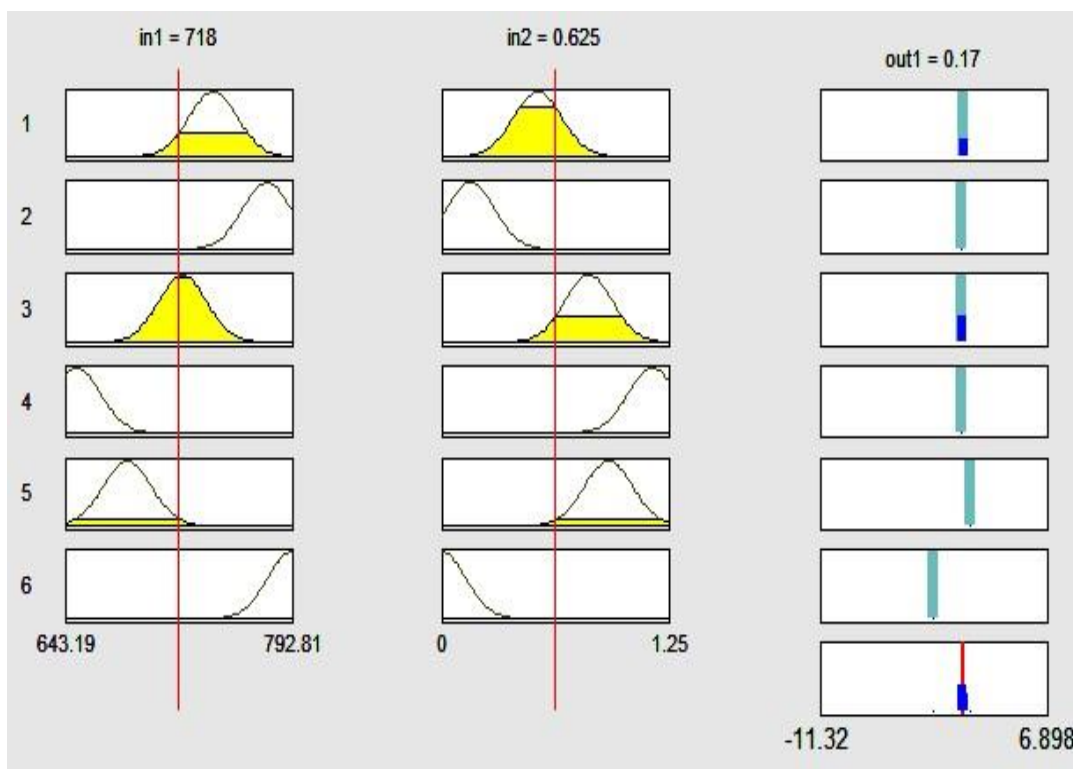
Figure 6. The inferred rules by the ANFIS using6fuzzy sets designed in Matlab software
