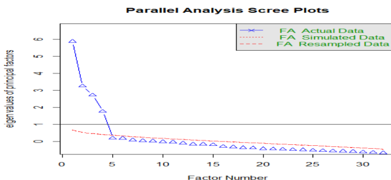
Figure 2. Optimum Number of Factors to be Extracted Using Resampling
