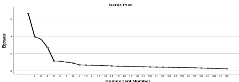
Figure 1. Optimum Number of Factors to be Extracted for the TI
