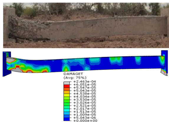
Fig. 7 Correlation of the results related to the distribution of tensile damage and failure occurred in the laboratory sample and finite element model
