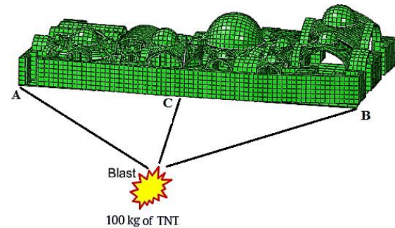
Fig. 12 Loading an explosion on Sheikh Baha'i's bath
