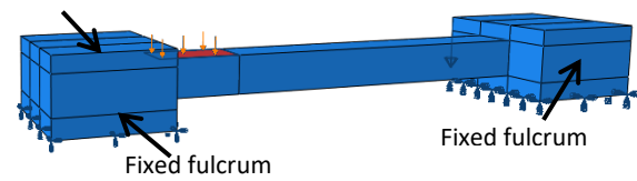
Fig. 5 Construction of boundary conditions and loading for reinforced concrete member
