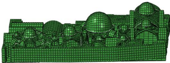
Fig. 8 Model made of bathroom in Abaqus environment
