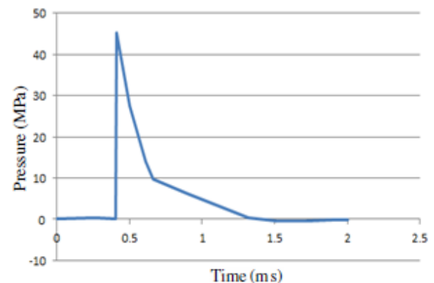
Fig. 3 Load applied to the column[8]
