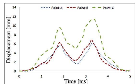
Fig. 13 Time history of the displacement under explosion
