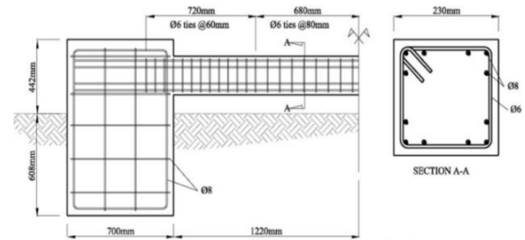
Fig. 1 General shape and specifications of laboratory sample [8]
