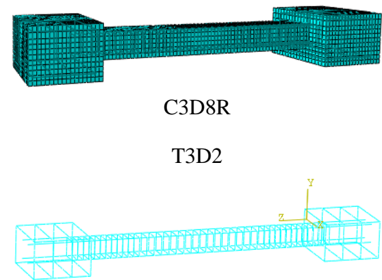
Fig. 6 Model comparison
