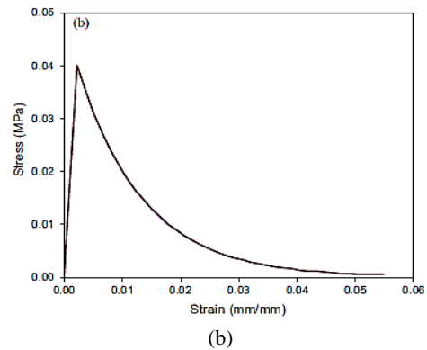
Fig. 9 Stress-strain curve of brick materials: (a) stress-compressive strain, (b) tensile-strain stress [12]
