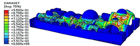
Fig. 11 Distribution of tensile damage of the bath in the final loading step
