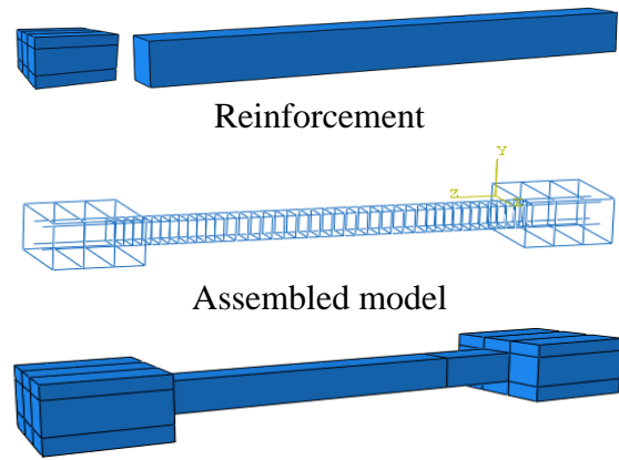
Fig. 4 Model assembly process
