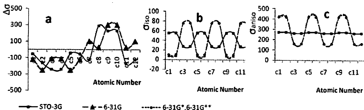
Fig. 3. The graphs of a) \Delta\sigma shielding values, b) isotropic shielding values ( \sigma_{iso} ), c) anisotropic shielding values ( \sigma_{aniso} ), of propose atoms of nanotube in gas phases at the HF, level with the STO-3G, 6-31G, 6-31G*,6-31G** basis sets in GIAO method.
