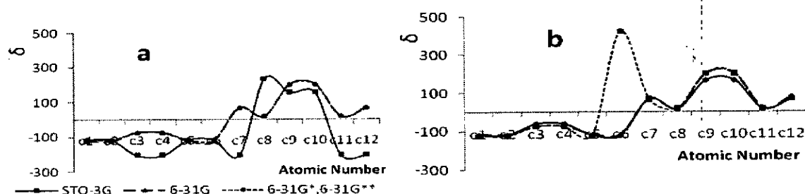
Fig. 2. Comparing of \delta shielding values at the HF, level with the STO-3G, 6-31G, 6-31G*, 6-31G** basis sets in GIAO method between a) gas and b) solvent phases.
