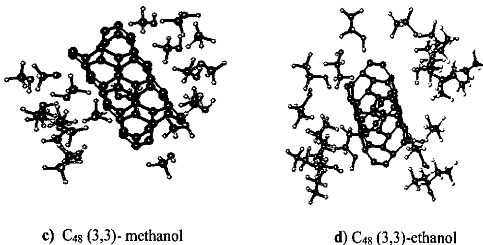
Scheme 1. Optimized structure of nanotube in different media.
