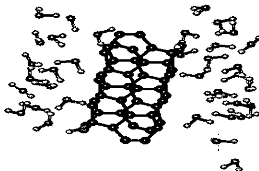
b) C 48 (3,3)-water
