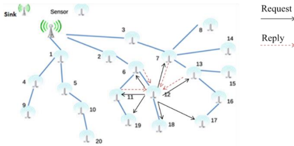
Figure 2. Protocol routing details
