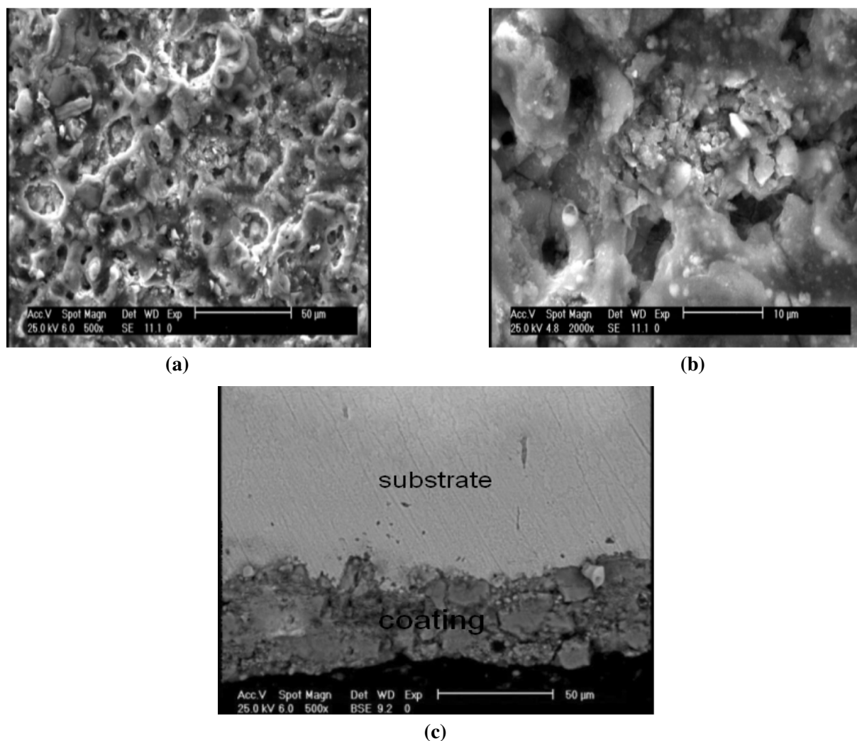
Fig. 2. (a) and (b) SEM pattern of surface morphology in 50 \mu m and 10 \mu m and (c) cross section of sample was coated through PEO process in carbonate solution.
