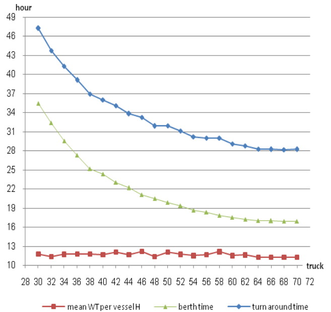
Fig. 13. Vessel's turnaround time
