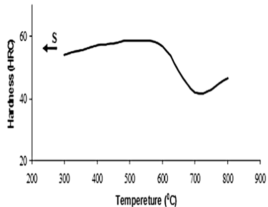
Fig. 2. The alloy hardness vs. different aging temperature at constant time of 70 min.
