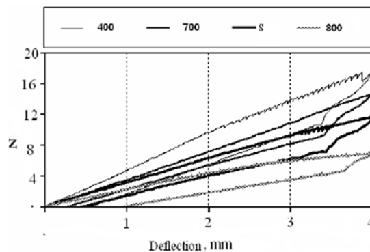
Fig. 7. Load-deflection curves of 3-point bending test performed at 25 °C.
