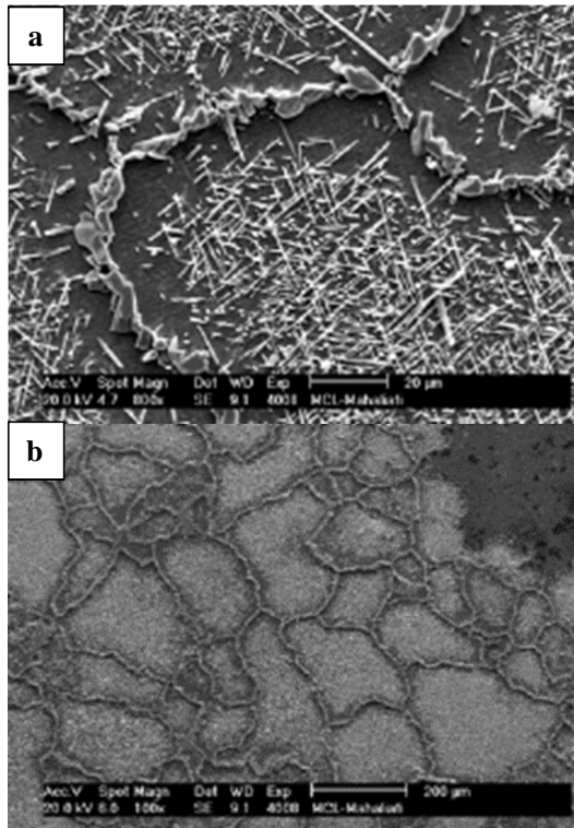
Fig. 4. a. SEM image of alloy aged at 400 °C for 8 h, b. magnified image.
