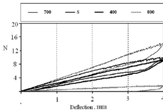
Fig. 8. Load-deflection curves of 3-point bending test performed at 60 °C.
