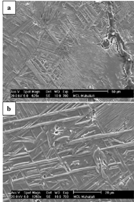
Fig. 6. a. SEM image of alloy aged at 700 °C for 70 min, b. magnified image.
