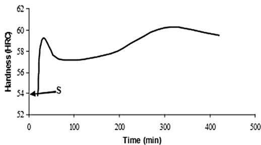
Fig. 1. Hardness vs. different aging time at constant temperature of 400 °C.
