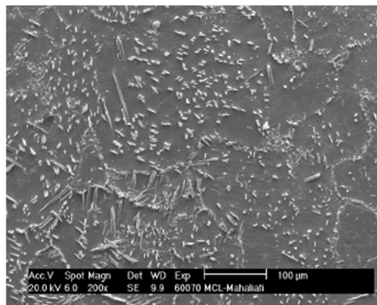
Fig. 5. SEM image of alloy aged at 600 °C and aging time of 70 min.
