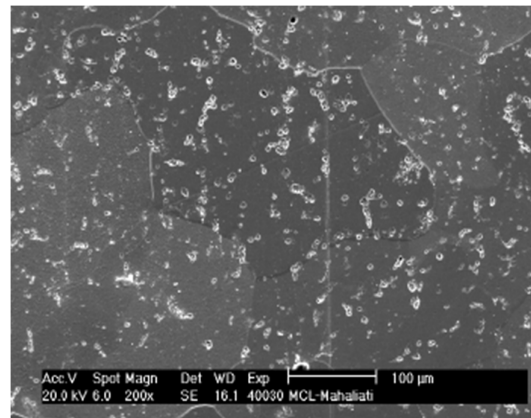
Fig. 3. SEM image of alloy aged at 400 °C for 30 min.
