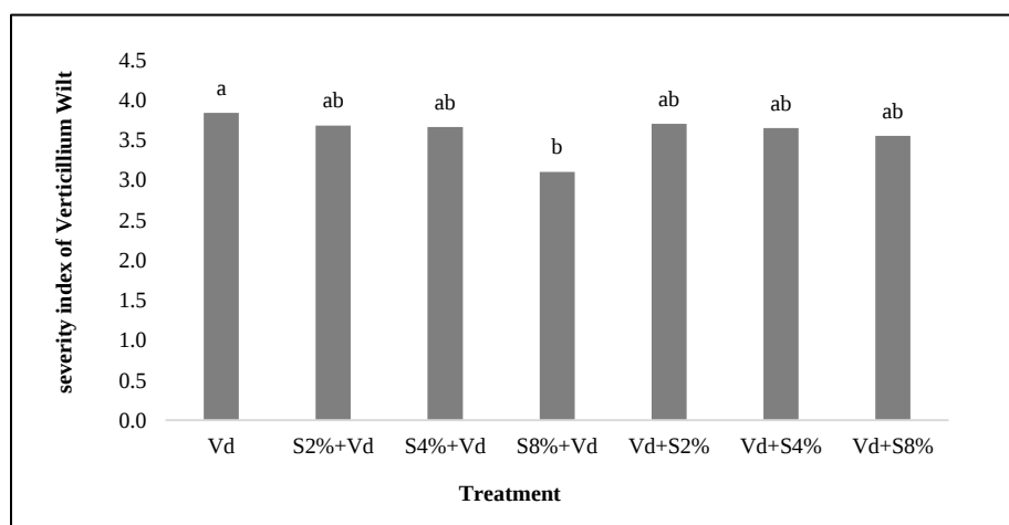
Figure 2. The severity index of Verticillium wilt of pistachio seedlings in treatments of mineral sulfur before and after inoculation with the pathogen. Means with the same letter are not significantly different according to Duncan's multiple range test ( P < 0.05 ). Vd: Verticillium dahliae . S2%, S4% and S8%, respectively, the concentrations of 2%, 4% and 8% of mineral sulfur.
