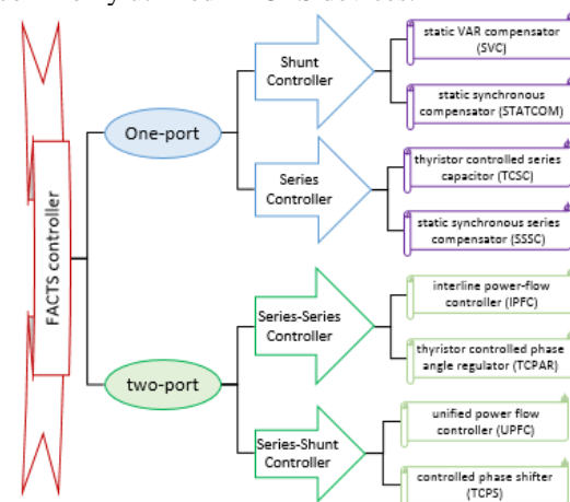
Fig. 2. The categorization of FACTS devices according to their connection type
