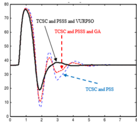
Fig. 14. Compare the answer rotor angle of generator 1
