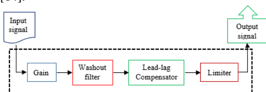
Fig. 1. Structure of conventional power system stabilizer
