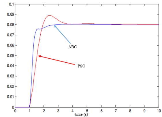
Fig. 20. Rotor angle changes to tuning TCSC parameters in two algorithms
