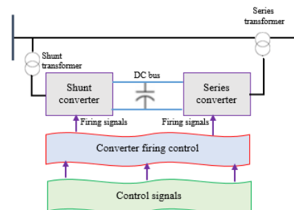
Fig. 8. UPFC basic configuration arrangement
