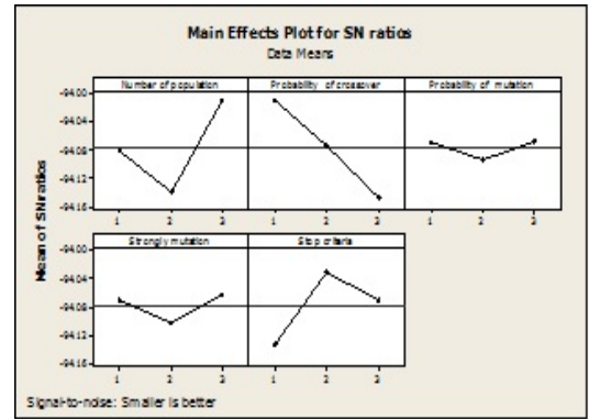
Figure 6: SN ratios for the GA algorithm.
