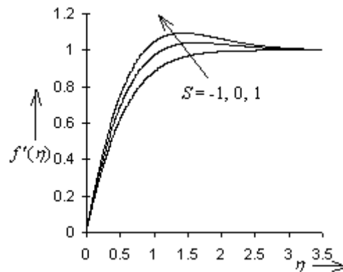
Fig. 2. Velocity distribution versus \eta when G_T = 1.0, G_C = 0.5, K = 0.0, Pr = 1 and Sc = 0.5 .
