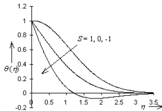
Fig. 6. Temperature distribution versus \eta when G_T = 1.0, G_C = 0.5, K = 5.0, Pr = 1 and Sc = 0.5 .
