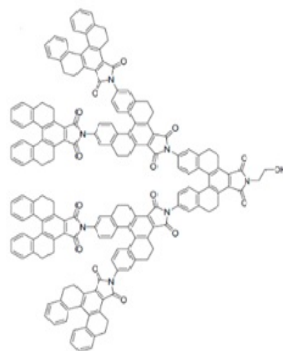
Figure 10: Helicene-based dendrimers, H [2]
