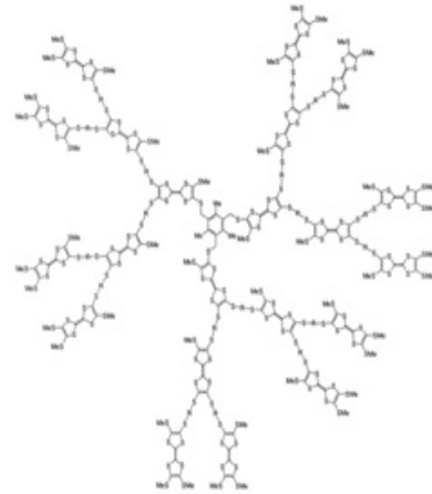
Figure 13: Tetrathiafulvalene [TTF] 21 -glycol dendrimer, T [3]
