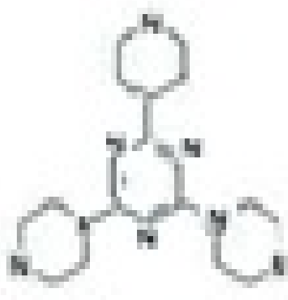
Figure 7: Polymer dendrimer, P [2]
