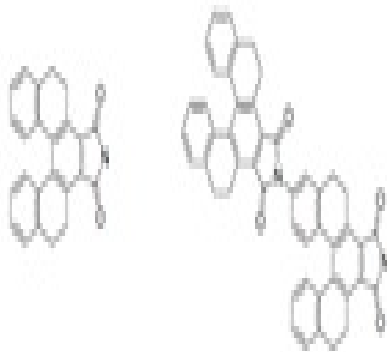
Figure 12: G_1 and G_2
