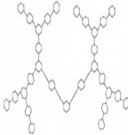
Figure 1: First-type nanostar dendrimer, NS_1[2]
