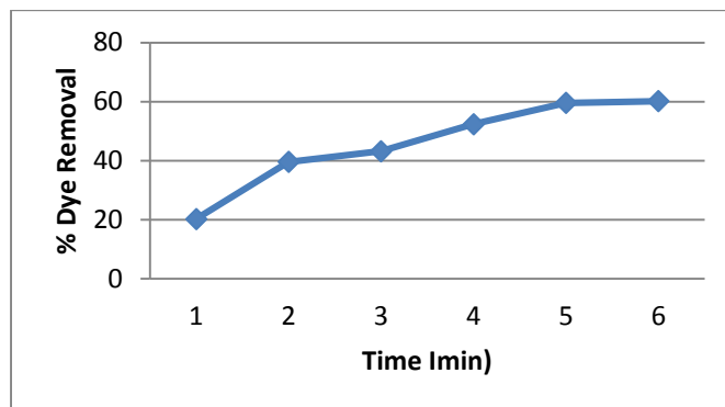
Fig. 6. Effect of contact time for 8 ppm red carmoisine concentrations; pH 4, 25 °C, agitation rate of 180 rpm and 0.733 g adsorbent in 150 ml of dye solution.
