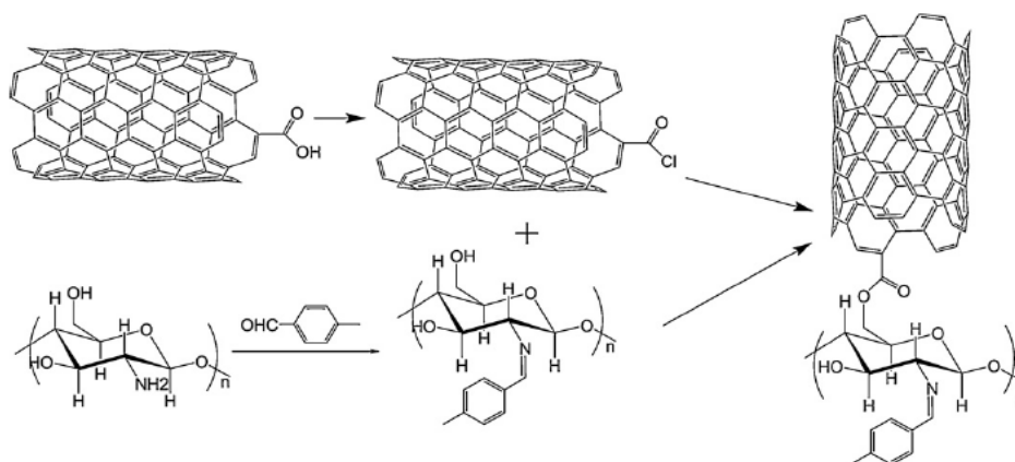
Figure 1: Schematic of Synthesis and structure of S-CS-MWCNTs.
