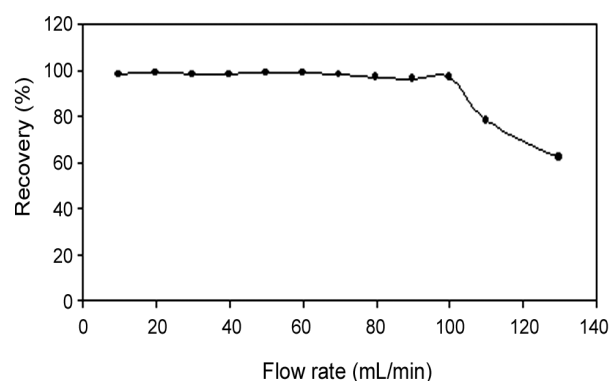
Figure 3: The effect of the flow-rate on extraction percent of Cu (II).
