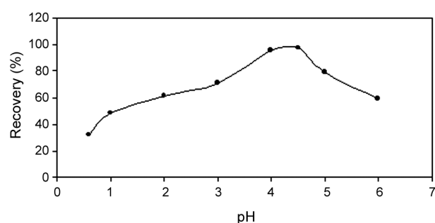
Figure 2: Influence of sample pH on the percentage recovery of Cu (II).
