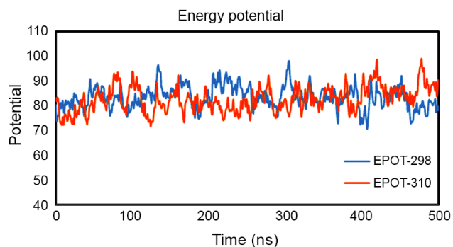
Fig. 2. The potential energy diagram, Monte Carlo simulation at 298 K and 310K.
