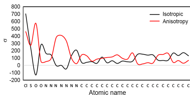
Fig. 3. NMR parameters of Dasatinib at the B3LYP/6-31G basis sets.
