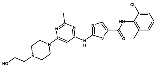
Fig. 1. Structure of Anticancer Dasatinib
