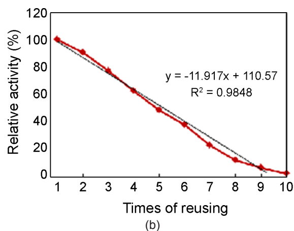
Fig. 5. Assessment of the stability of immobilized laccase enzyme (A) and re-usability (B).
