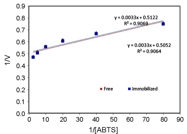
Fig. 3. Lineweaver-Burk diagram to determine the parameters of K_m and V_m of free and immobilized laccase enzymes.
