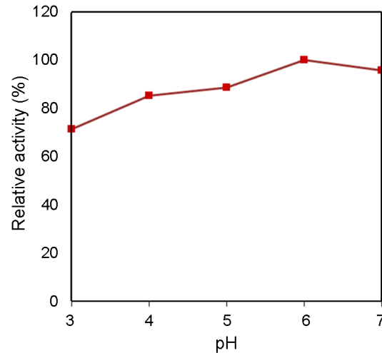
Fig. 2. Investigation of the effect of pH on the process of immobilization of the laccase enzyme on porous zinc oxide nanoparticles.
