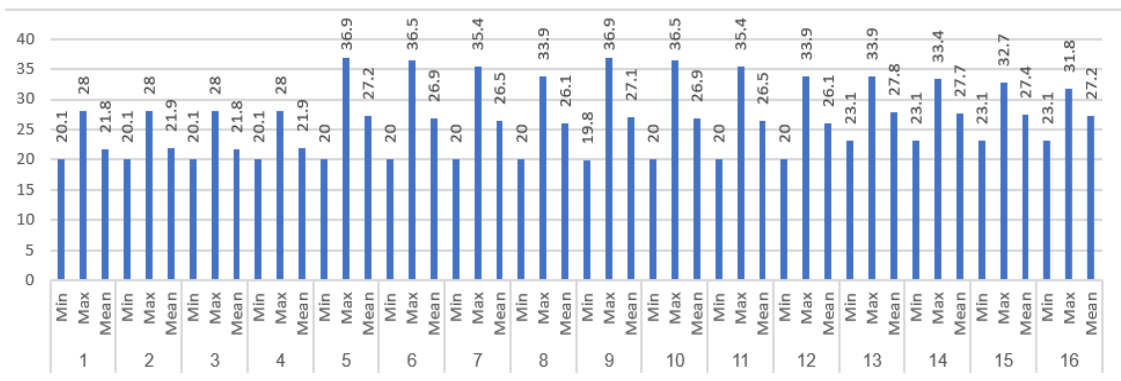
Fig. 17: Graph comparing indoor air temperature between simulated samples
