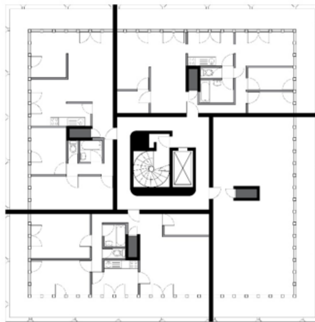
Fig. 3: The Montereau project. The Project Designer: Les frerez Arsene henry. 1971 France (Source: Thaniyabadi et al., 2017 )
