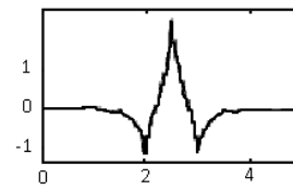
Coiflet wavelet (Coif1)
