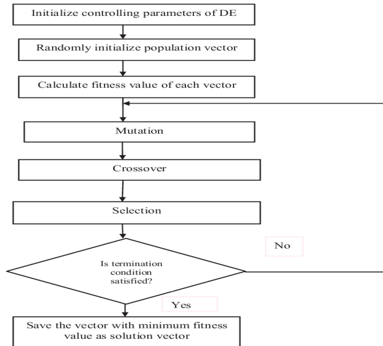
Fig.1: Flowchart of the Differential Evolution Algorithm [30]
