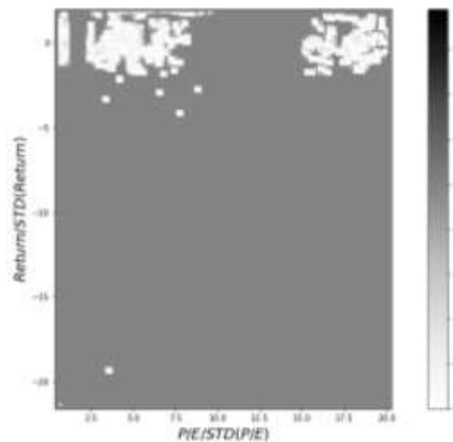
Fig. 7: The joint quantum potential in chemical market
