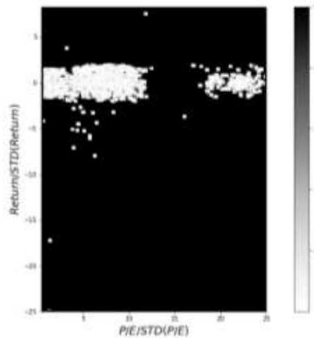
Fig. 6: The joint quantum potential in Metal market
