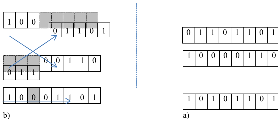
Fig. 2: Genetic operators a) Crossover b) Mutations
