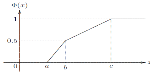
Fig. 1: Zigzag Uncertainty Distribution
