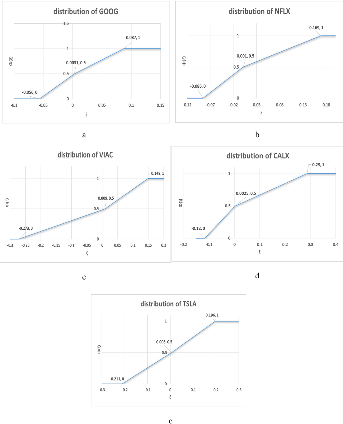
Fig. 2: Zigzag Uncertainty Distribution of (a) GOOG (b) NFLX (c) VIAC (d) CALX (e) TSLA base on belief degree of experts.is a figure.
