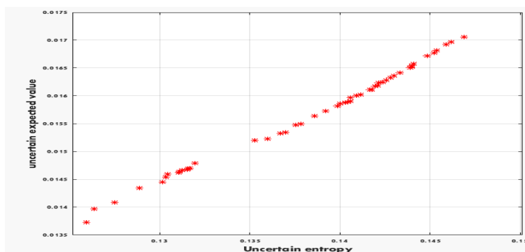
Fig. 3: Solutions of the Uncertain Mean-Entropy Portfolio Optimization For The Mopso
