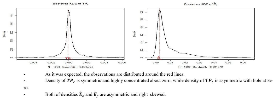
Fig. 3: The KDEs of \hat{E}_c (left panel) and TP_c (right panel).
