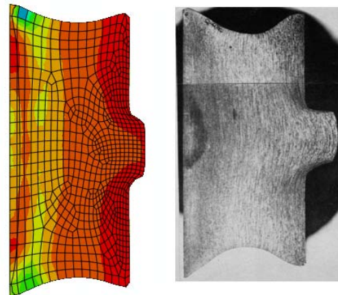
Fig. 2 Comparison between the simulated and experimental ring
