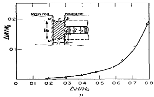
Fig. 3 Comparison between the a) simulated and b) experimental spread vs total reduction in wall thickness, center spread
