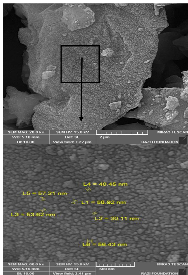
Fig. 8 FE-SEM images taken from the nanocomposite powder after its calcination in an oven under Argon atmosphere for 30 min and at a temperature of 1250\text{ }^\circ\text{C}
