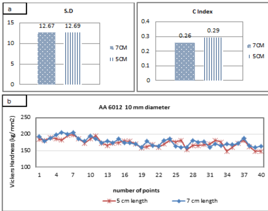
Figure 7. a) S.D and C index values of measured micro hardnesses b) the profile of micro hardness in the cross section of the AA6012 samples with \phi = 10\text{mm} and lengths of 70 and 50 mm
