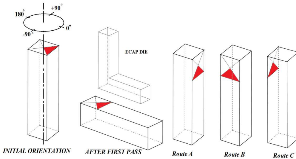
Figure 2. Four fundamental routes [41]
