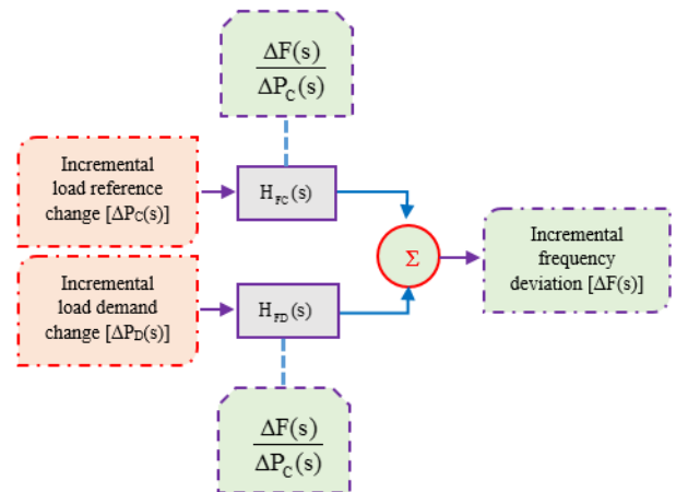
Fig. 2. Representation of a single-area power system based on transfer functions
