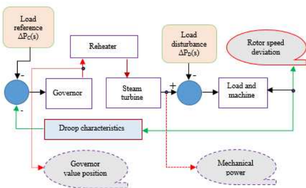
Fig. 1. Production unit structure with steam reheat turbine
