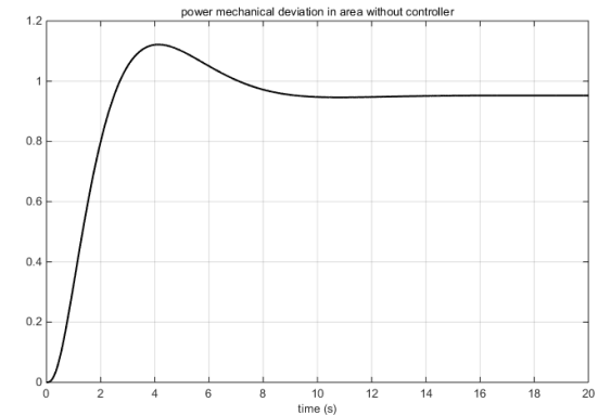
Fig. 4. Power mechanical deviation in power system without controller
