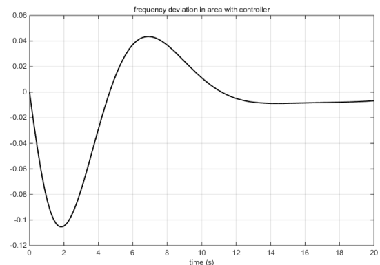
Fig. 5. Frequency deviation in power system with controller
