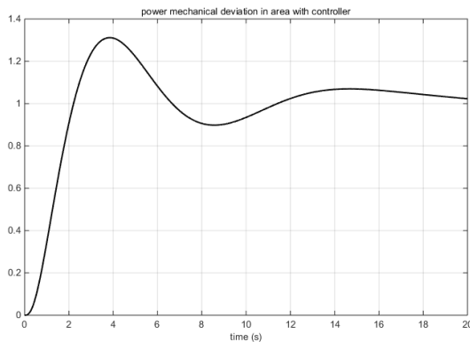
Fig. 6. Power mechanical deviation in power system with controller
