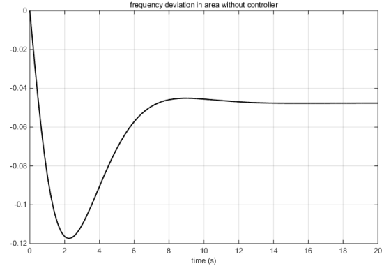
Fig. 3. Frequency deviation in power system without controller
