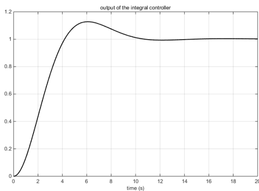
Fig. 7. Integral controller output system with controller
