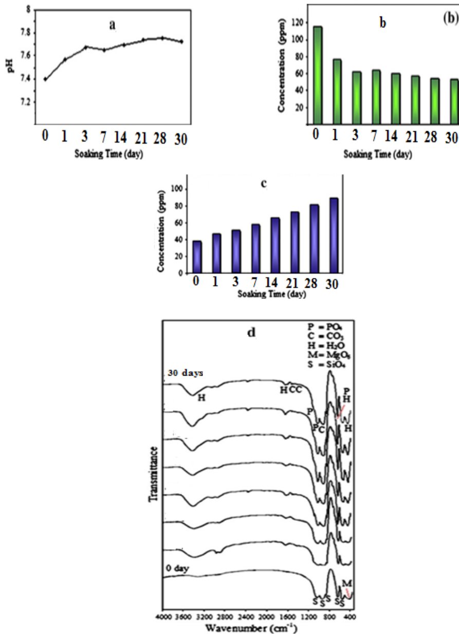
Fig. 2. The variations of (a) pH, (b) Ca, and (c) Mg ions concentration of the simulated body fluid, after soaking the nanostructure DS ceramics and (d) FTIR spectra of nanostructure DS soaked in the SBF for different periods of time.
