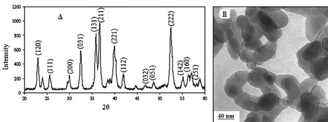
Fig. 1. (A).X-RAY diffraction pattern and (B) Transmission electron microscopy (TEM) image of obtained diopside powder after 10 h mechanical activation
