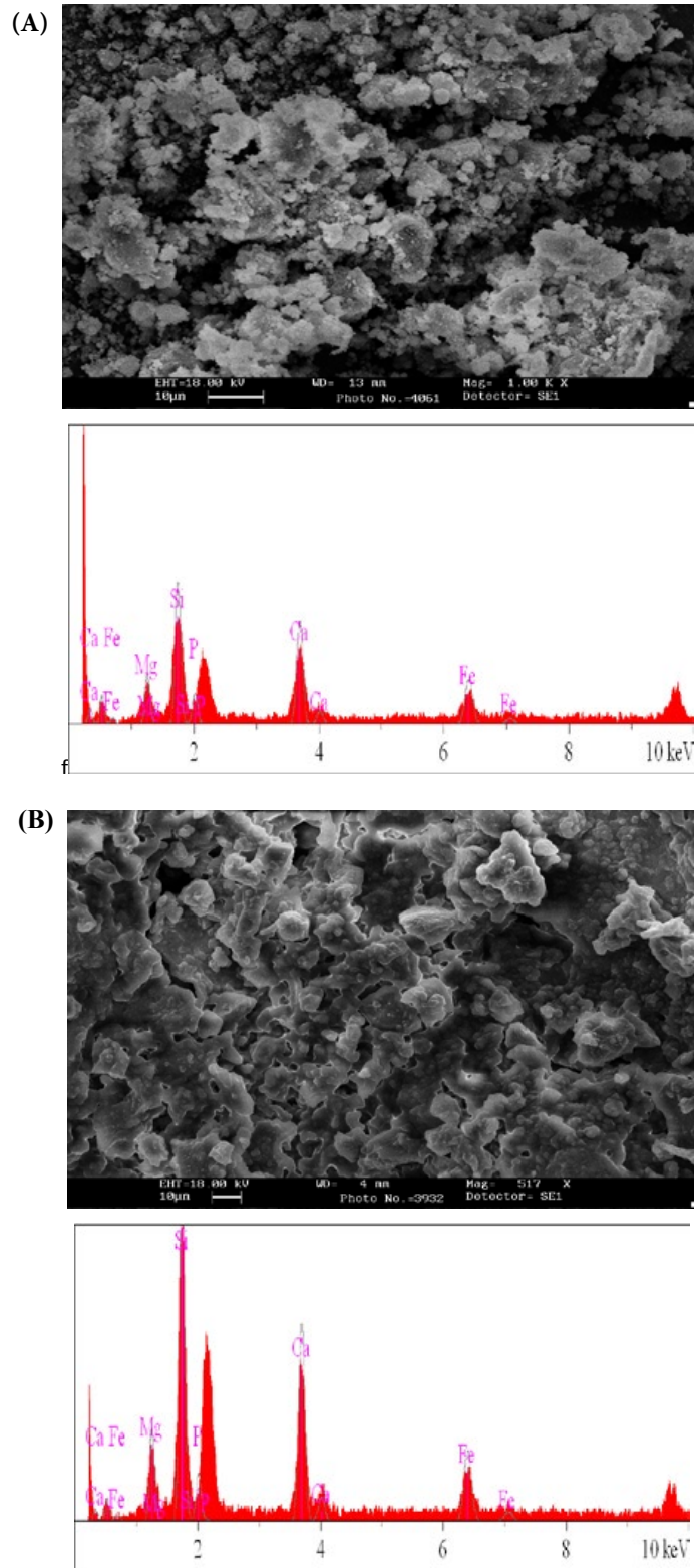
Fig. 3. SEM micrographs and EDS spectra of the surfaces of nanostructure DS after immersion in SBF for (A) 14 days and (B) 30 days.
