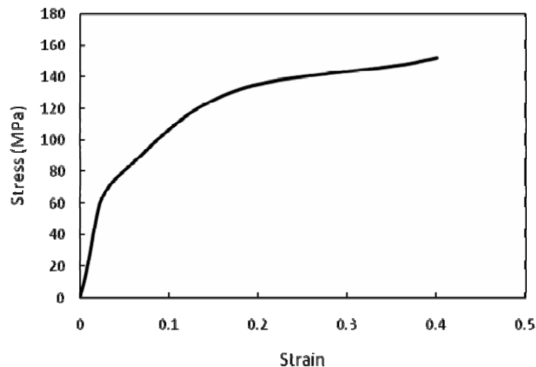
Fig. 3. Stress-strain curve of AZ91 at 300° C [14]
