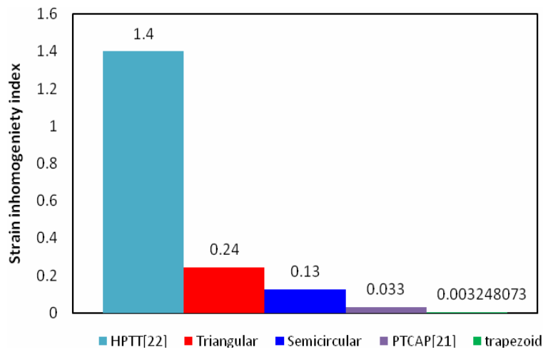
Fig. 6. Strain inhomogeneity index in three channel types compared to other SPD methods
