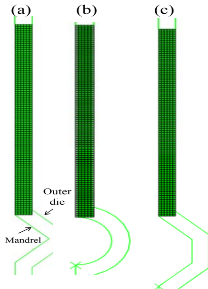
Fig. 4. FEM model and meshed tube cross section in the (a) triangular, (b) semicircular and (c) trapezoidal channels
