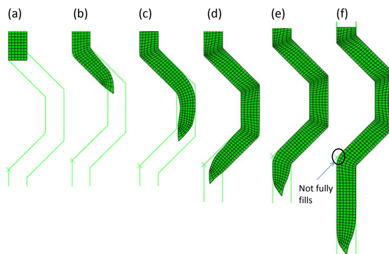
Fig. 9. The material flow and deformation geometries during different stages of the TCAP processing with trapezoidal channel geometry
