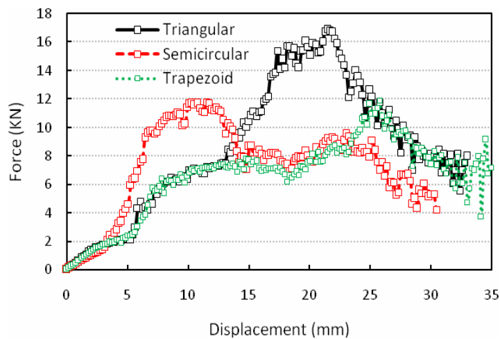
Fig. 7. FE calculated processed load in TCAP processing with trapezoidal channel geometry compared to triangular and semicircular channels
