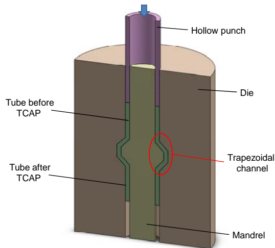
Fig. 1. Schematic of the tubular channel angular pressing (TCAP) using trapezoidal channel
