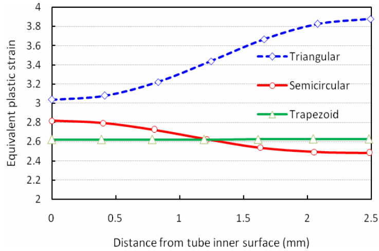
Fig. 5. Path plot of the equivalent plastic strain through the thickness, from inside to outside, for trapezoidal channel compared to other cases (The paths are indicated by arrows in Fig. 4(d-f).)
