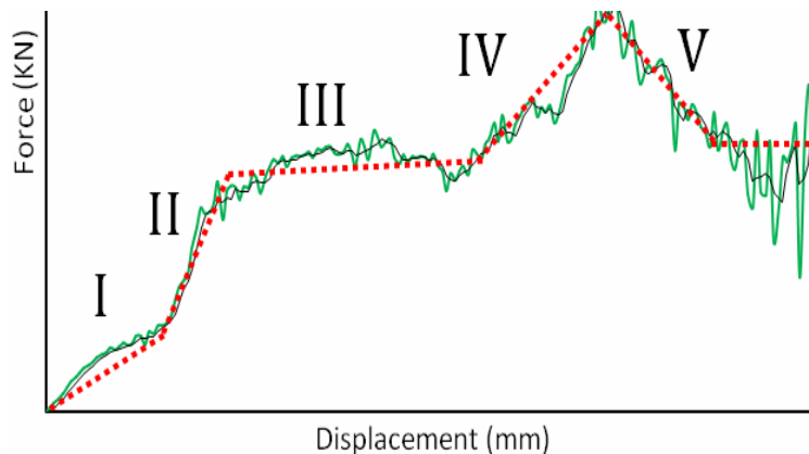
Fig. 8. Load-displacement diagram in the TCAP process with the trapezoidal channel geometry
