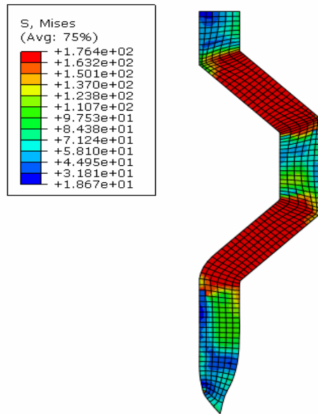
Fig. 10. FEM predictions of the effective stress contour during the TCAP processing with trapezoidal channel geometry
