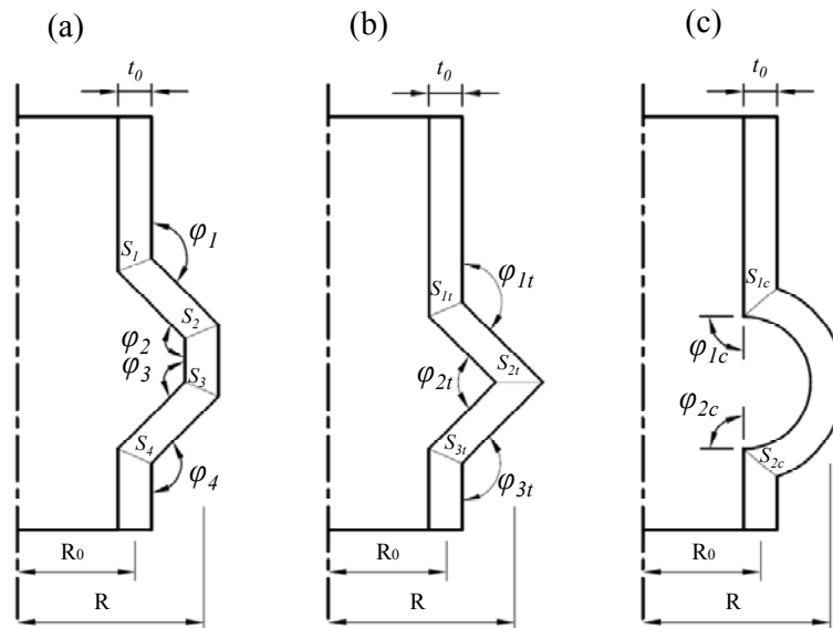
Fig. 2. Processing parameters in the TCAP processing using (a) trapezoidal, (b) triangular and (c) semicircular channel geometries (Curvature angles were considered equal to zero.)
