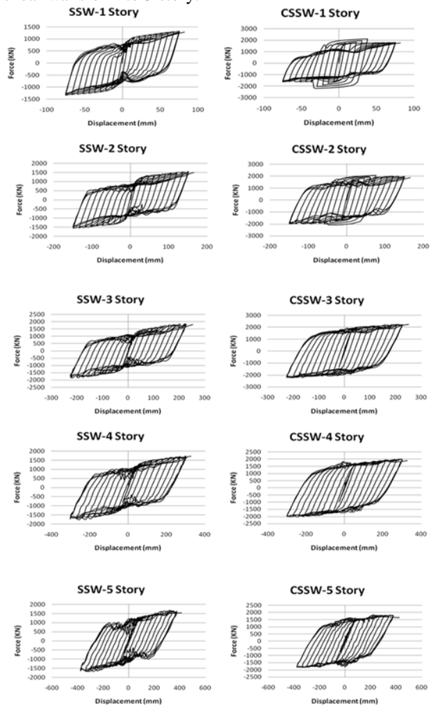
Figure 5. Hysteresis curves of steel and composite shear walls for 1 to 5 story
