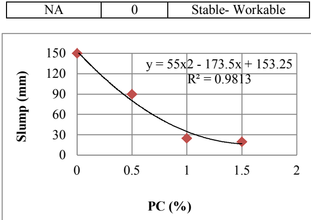
Figure 3. Effects of the PC on the workability of the fresh concrete
