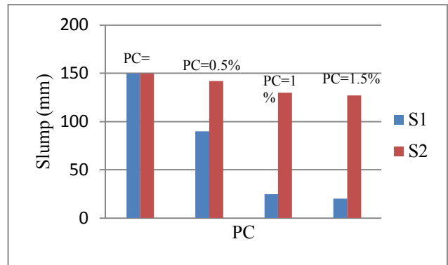
Figure 4. The comparison of the slump of samples before and after adding the superplasticizer
