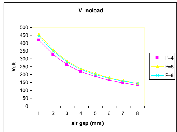
Fig. 9. Output voltage (no-load) (V) vs. air gap (m)
