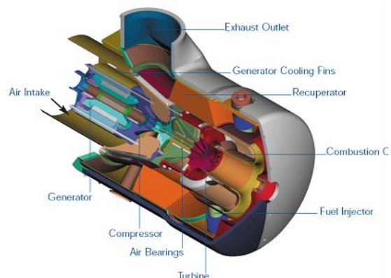
Fig.1 View of a Capstone microturbine [3]
