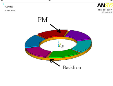
Fig. 5 View of a rotor of HSAFG
