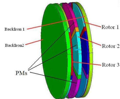
Fig. 3 Side view of high-speed axial-flux generators
