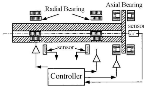
Fig. 7 Magnetic bearing
