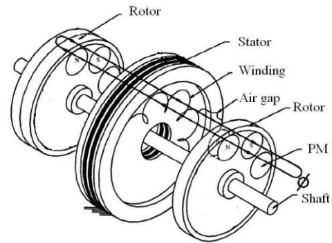
Fig. 6: Representation of a winding of stator of HSAFG
