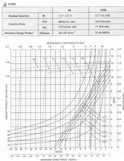
Fig. 4 Curves of N35H used in this machine
