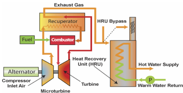
Fig. 2 Cogeneration System (CHP)
