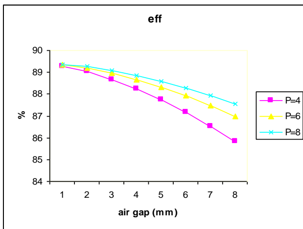
Fig. 11. Efficiency (%) vs. air gap (m)
