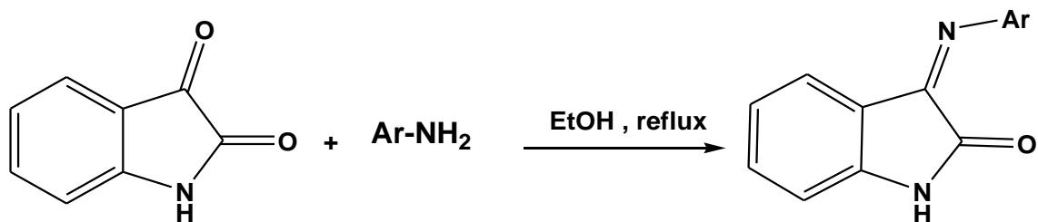
Figure 1. Schematic representations of synthesized isatin schiff bases
