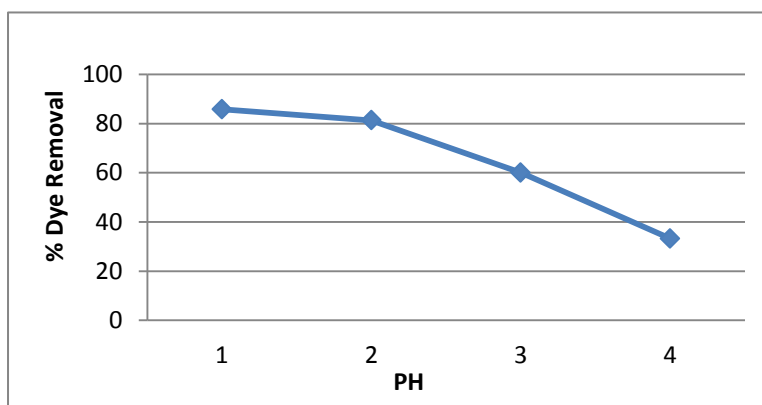
Fig 3. Effect of pH on the removal of erythrosine 25^\circ\text{C} , agitation rate of 1800rpm 0.733 gr adsorbent in 100 ml of 8 \text{ mg L}^{-1} dye solution
