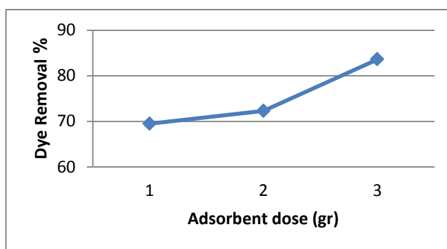
Fig (9): Effect of different copper oxide dose pH 4, 25^\circ\text{C} , agitation rate of 180 rpm and initial dye concentration 8\text{mg L}^{-1} in 150 ml of Erythrosine dye solution.
