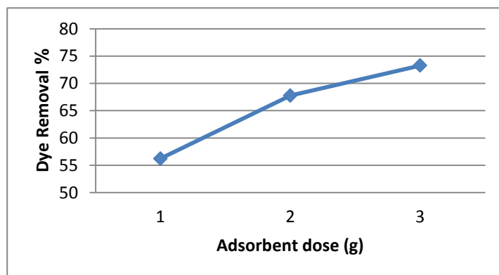
Fig (10): Effect of different copper oxide dose pH 4, 25^\circ\text{C} , agitation rate of 180 rpm and initial dye concentration 8\text{mg L}^{-1} in 150 ml of Red Carmoisine dye solution.
