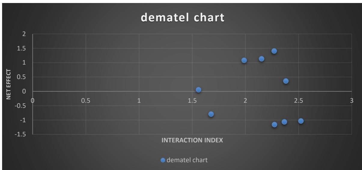
Fig.3: DEMATEL Chart
