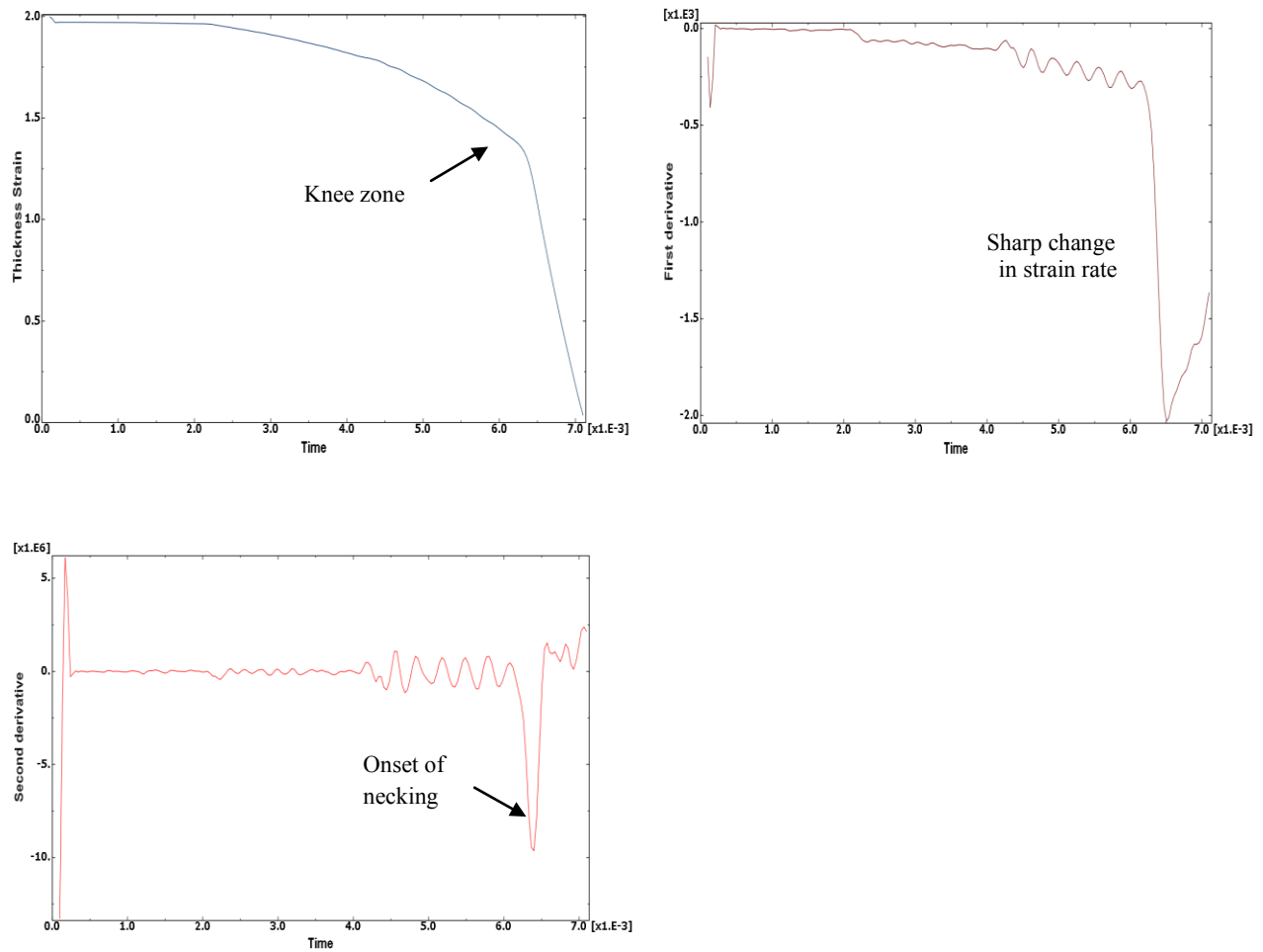
Fig.10 Thickness strain as a function of time and its derivatives for a particular specimen.
