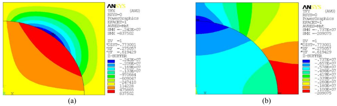
Fig.7 The heat flux: a) Q_x , b) Q_y in nodes at temperature ( T = 10^{-3}^{\circ}\text{C} ) on line y=1 and \xi = 0.504 .
