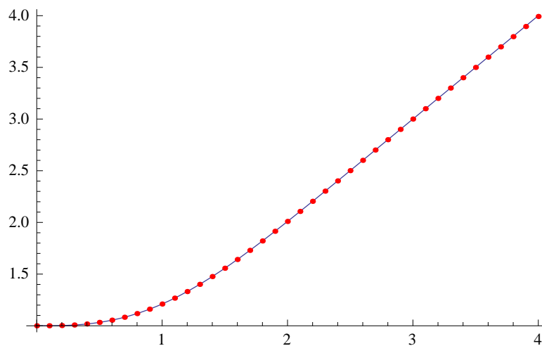
Fig. 2. he exact solution (solid) versus the approximate solution (bolded dash).
