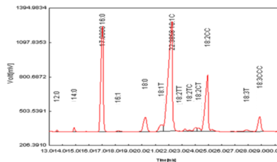
Fig. 2. Fatty acid profile of tallow stearin
