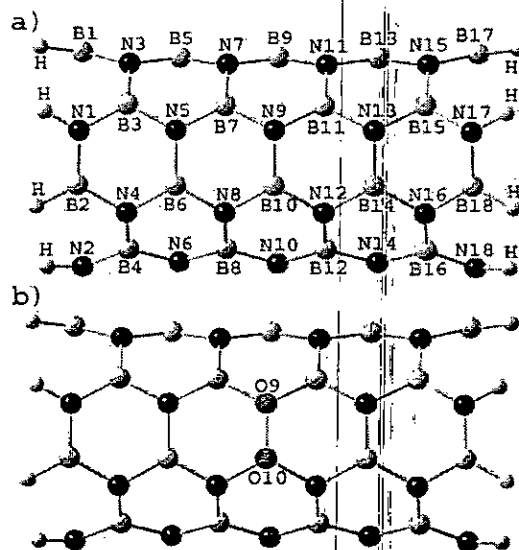
Fig. 1. To ease, 2D views of the models are shown. The original armchair model is shown in panel (a) and the impure armchair model is shown in panel (b).
