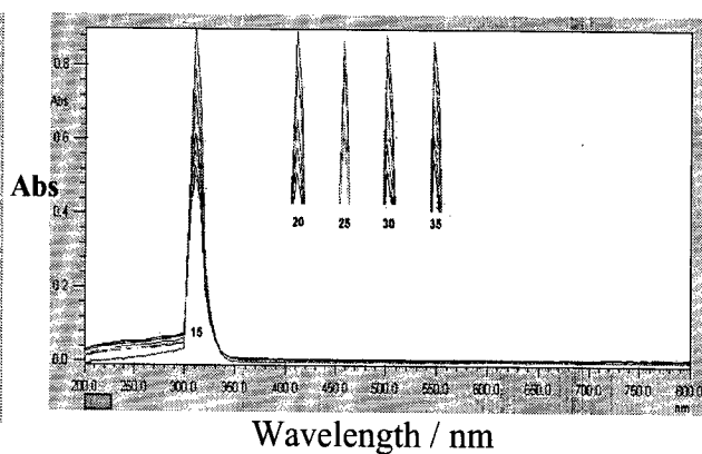
Fig.4. Absorption spectra of Fe^{2+}_{(aq)} upon titration with L-Alanine in potassium hydrogen phthalate buffer, pH 4.1, and ionic strength of 0.1M KNO_3 at 15°, 20°, 25°, 30° and 35 °C.
