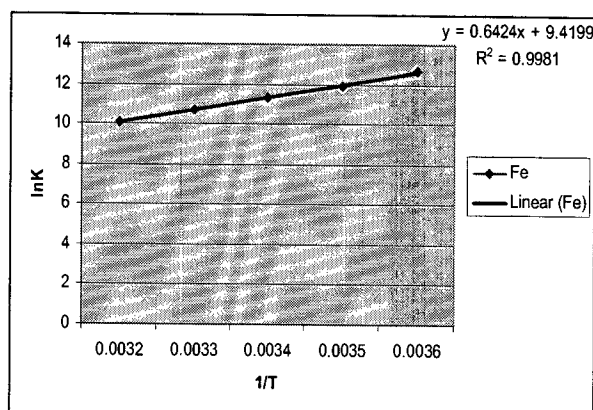
Fig.5. A linear plot of \ln K versus 1/T for binding of Fe^{2+}_{(aq)} to L-Alanine in the potassium hydrogen phthalate buffer, pH 4.1, and ionic strength of 0.1M KNO_3 .
