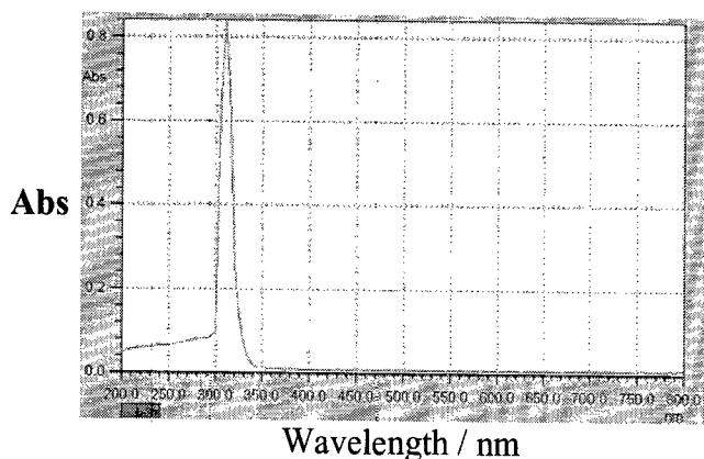
Fig.2. Absorption spectra of Fe^{2+}_{(aq)} and its maximum band.
