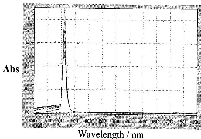
Fig.3. Absorption spectra of Fe^{2+}_{(aq)} upon titration with L-Alanine in potassium hydrogen phthalate buffer, pH 4.1, and ionic strength of 0.1M KNO_3 at 25 °C
