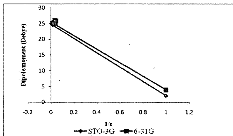
Fig. 2. Plot of the \mu (Debye) versus the 1/\epsilon , obtain from the (LanL2DZ+STO-3G) and (LanL2DZ+6-31G) calculations for \text{Sn}(\text{CH}_3)_2(\text{NAC}) - \text{CNT} Complex.
