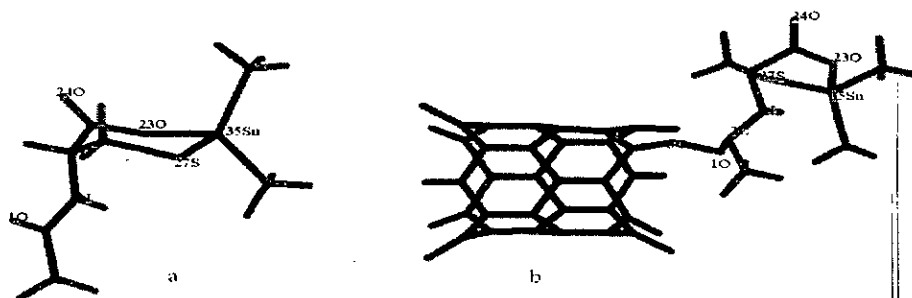
Fig. 1. Optimized geometries of the Sn (CH 3 ) 2 (NAC) (a) and (Sn (CH 3 ) 2 (NAC) - CNT complex (b) obtained at the (LanL2DZ+6-31G) level.
