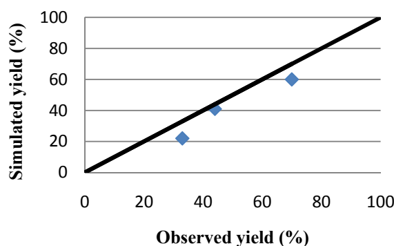
Fig. 2: Observed versus simulated relative yield for winter wheat
