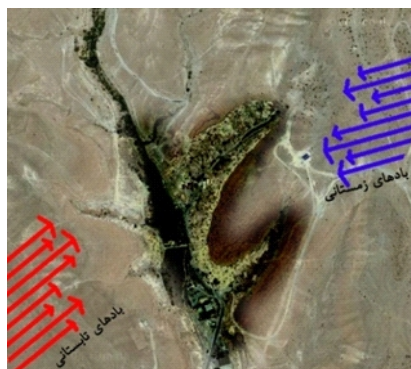
Fig. 3: Building orientation in Meymand, Kerman Right: Building orientation, Left: Prevailing wind in summer and winter
